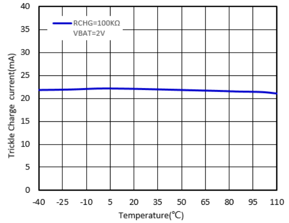
Trickle Charge Current vs Ambient Temperature
